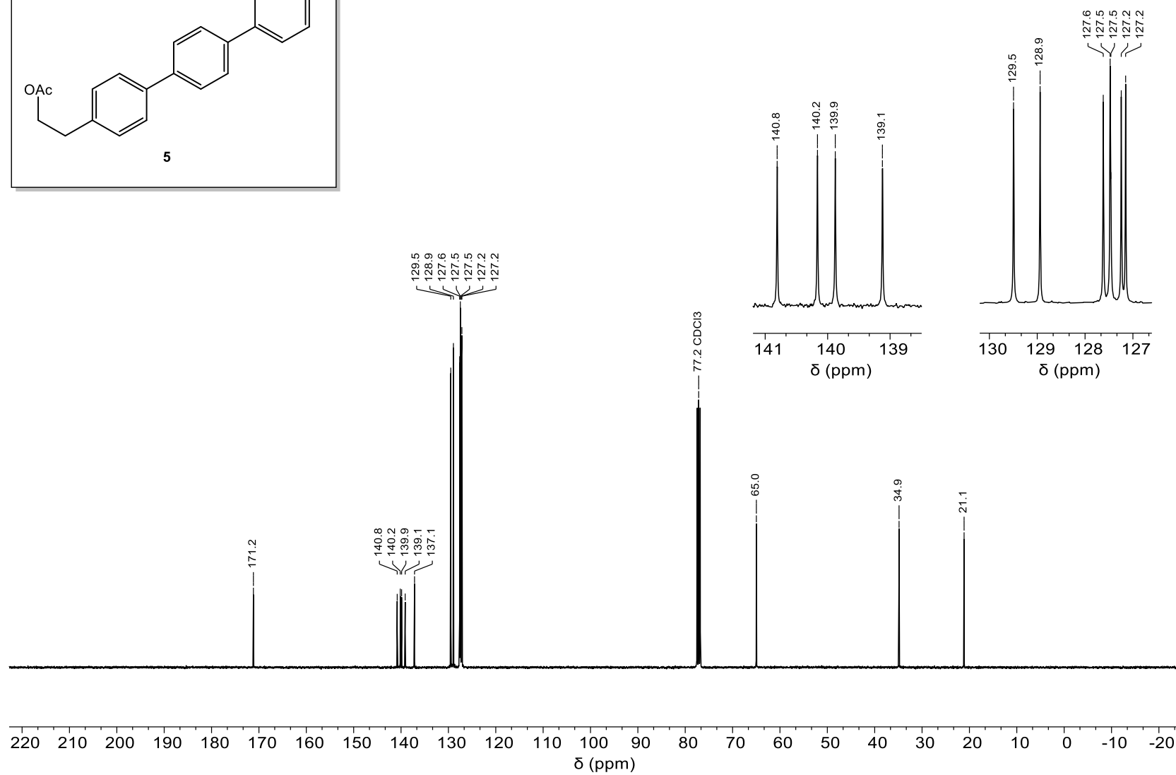
13 C NMR (101 MHz, CDCl 3 ) of [4-(4-phenylphenyl)phenyl] ethyl acetate (5).
